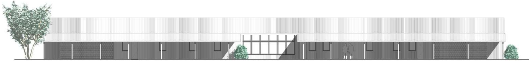
2 Front Elevation 1:100
